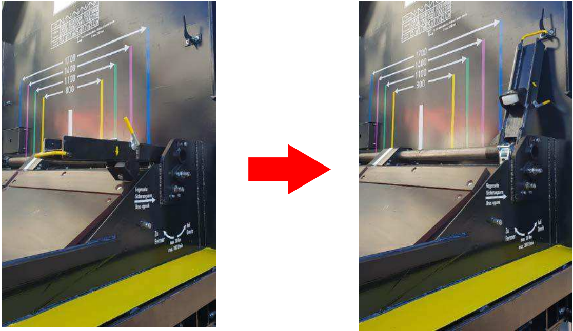
Figure 16 Positioning the arm on the front wall
