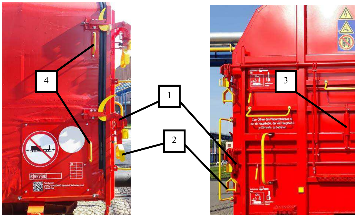
Figure 1 Mechanism for locking tarpaulin
